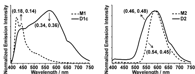
Figure 2. Emission spectra of molecules M1 , D1c , M2 , and D2 in the solid state with CIE coordinates under excitation at 365 nm.
